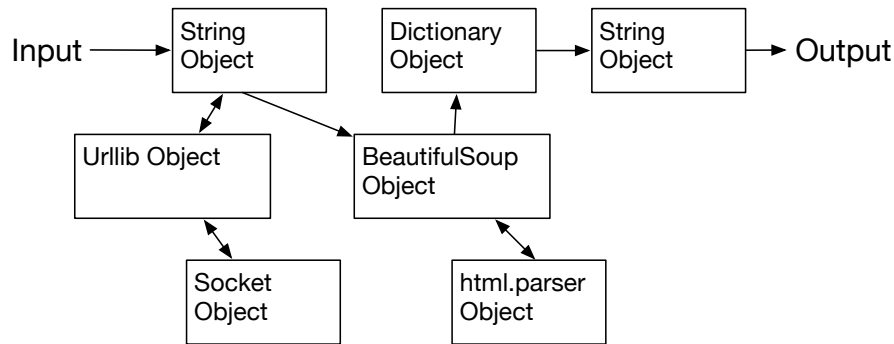
Figure 14.2: A Program as Network of Objects
