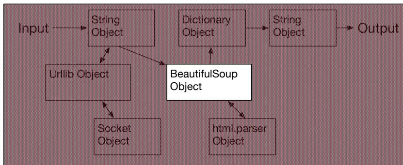
Figure 14.4: Ignoring Detail When Building an Object
