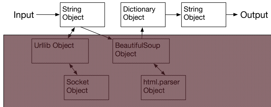
Figure 14.3: Ignoring Detail When Using an Object
