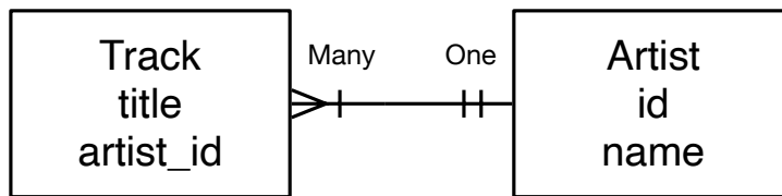
Figure 15.4: A Verbose One-to-Many Data Model
