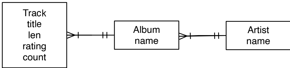
Figure 15.6: Tracks, Albums, and Artists
