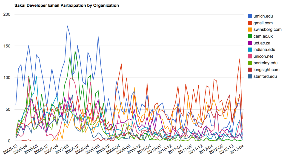
Figure 16.4: Sakai Mail Activity by Organization
