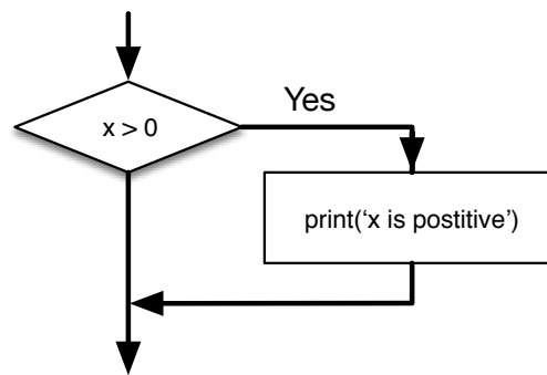
Figure 3.1: If Logic
