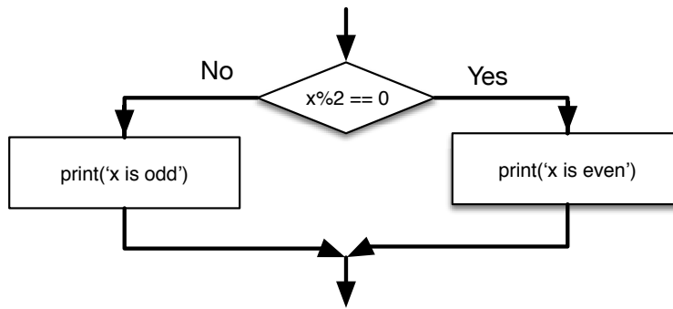
Figure 3.2: If-Then-Else Logic
