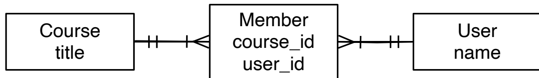
Figure 15.8: A Many to Many Connector Table
