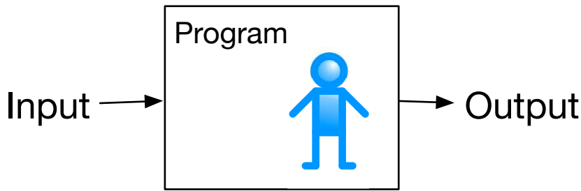
Figure 14.1: A Program
