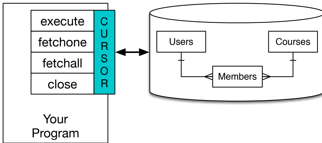
Figure 15.2: A Database Cursor
